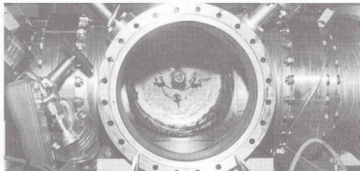
Interior of a CVD chamber used in the deposition of diamondlike films in Dr. O'Brien's laboratory
